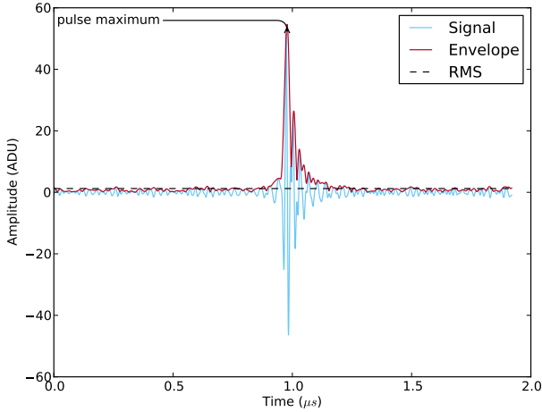
Fig. 16. The solid light line shows the up-sampled signal. Overlaid is the Hilbert envelope and the RMS noise in black dashes. A pulse is accepted whenever the signal to noise ratio exceeds three.
